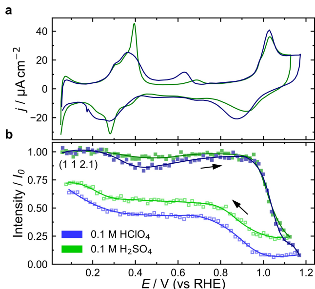
Figure 1. Oxidation and reduction in 0.1 M \text{H}_2\text{SO}_4 and 0.1 M \text{HClO}_4 electrolyte. a) Cyclic voltammograms and b) corresponding X-ray intensity at (1\ 1\ 2.1) in 0.1 M \text{H}_2\text{SO}_4 and 0.1 M \text{HClO}_4 . The electrochemical and structural data were simultaneously recorded at 20 mV/s and indicate that formation of the surface oxide above 0.98 V proceeds in an identical manner. The solid lines in b) serve as a guide to the eye. The data in 0.1 M \text{HClO}_4 has been published previously in Ref. [23].
