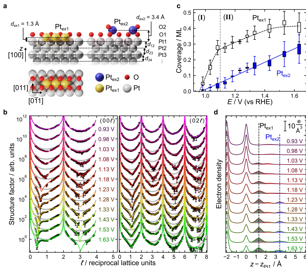
Figure 2. Atomic-scale structure of the stripe-like and amorphous oxide phases. a) Schematic illustrations of the two Pt oxide phases. On the left, top and side views of the geometry of the \text{Pt}_{\text{ex1}} in the stripe oxide are shown; the right side provides a side view of the \text{Pt}_{\text{ex2}} extraction site. Arrows indicate fitted vertical distances ( d ) between interface species. All other fit parameters and the best-fit parameter values are summarized in Table S2. b) Specular CTR ( 00\ell ) and one of the six measured non-specular, non symmetrically equivalent CTRs at potentials from close to the onset of oxidation at about 1 V up to 1.63 V. The CTR data at each potential are offset by a factor of 8 with respect to each other and are shown together with fits (colored solid lines). As a reference, the CTR fit of the data close to the onset of oxidation at 0.93 V is shown as solid gray lines. The full set of the measured CTRs and the corresponding fits are shown in Figure S1. c) Potential-dependent coverage of the extracted Pt atoms in \text{Pt}_{\text{ex1}} sites and \text{Pt}_{\text{ex2}} sites. The stripe oxide and amorphous oxide growth regimes are marked with (I) and (II), respectively. Rectangular boxes indicate the systematic error caused by the ambiguity of the location of the \text{O}_{\text{ad}} layer. The error bars represent the standard uncertainties of the CTR fits as standard deviations. Further details on the error analysis are given in the Supporting Information. d) Electron density profiles along the surface normal corresponding to the CTR fits. The density profiles at different potentials are offset from each other by 10 \text{ e \AA}^{-3} . Black and blue dashed vertical lines indicate the location of the \text{Pt}_{\text{ex1}} and \text{Pt}_{\text{ex2}} extraction site, respectively.
